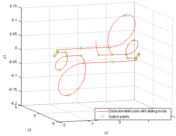
Figure 4: Clockwise trajectories of the system in (35) for a = 0.05 , b = 10 , d = 1 , s = -2 , and x_0 = [0.05 \ -0, 01 \ 0.1]^T : 3 - D view of the Periodic orbit of x_1 versus x_2 and x_3 .
