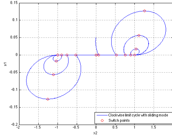
Figure 3: Clockwise trajectories of the system in (35) for a = 0.05 , b = 10 , d = 1 , s = -2 , and x_0 = [0.05 \ -0.01 \ 0.1]^T : The evolution of x_2 versus x_1 .
