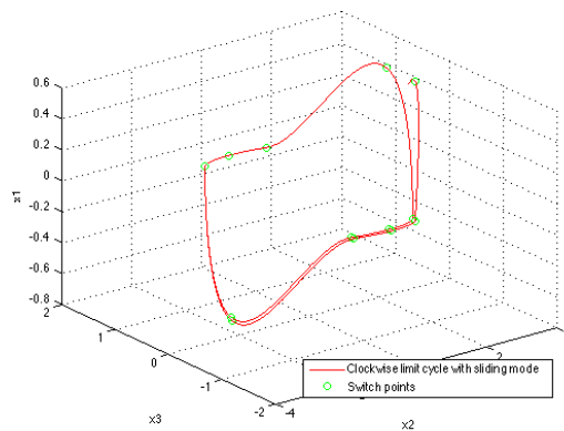
Figure 2: Clockwise limit cycle with \beta = 0.5 , and x_0 = [0.5 \ 3 \ 0.1]^T : 3D orbit of x_1 versus x_2 and x_3
