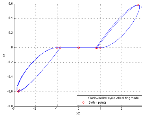
Figure 1: Clockwise limit cycle with \beta = 0.5 , and x_0 = [0.5 \ 3 \ 0.1]^T : x_2 versus x_1 .
