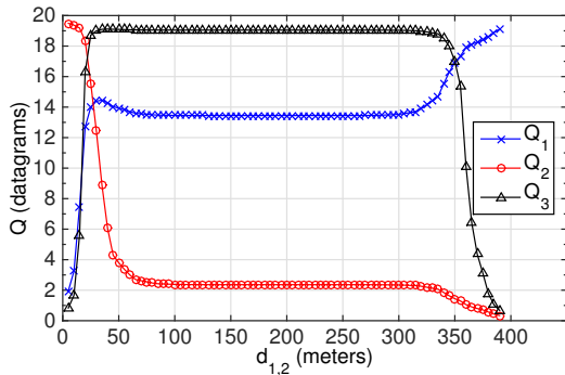
Fig. 9: Mean buffers occupancy as a function of the distance between nodes 1 and 2 with the workload level \Lambda^r = 2.5 Mb/s. K_n = 20 and \Lambda^r = 2.5 Mb/s.
