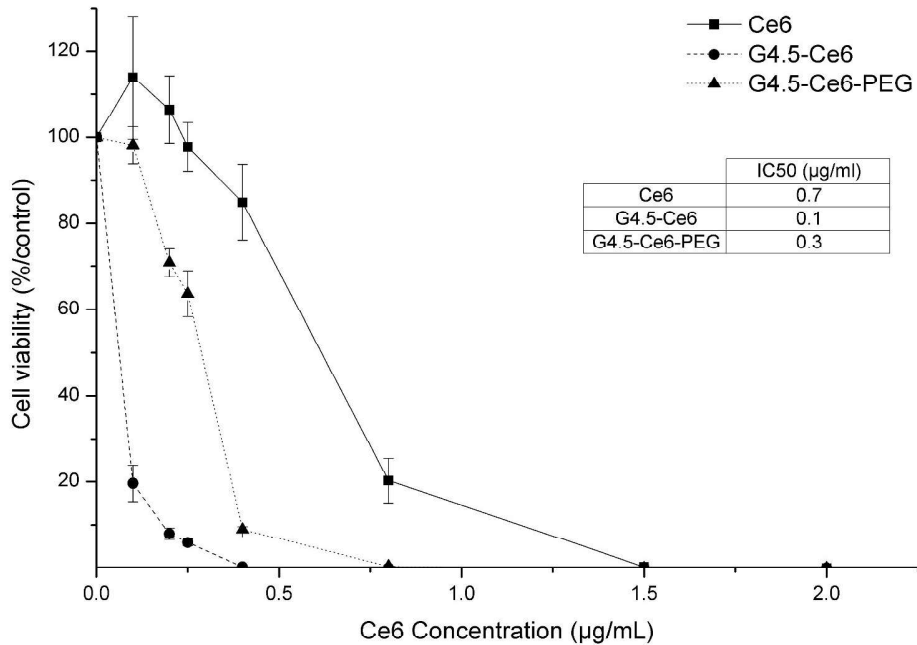
Fig. 2: In vitro antitumor activity of free Ce6 (square), G4.5-Ce6 (round) and G4.5-Ce6-PEG (triangle) after photoirradiation (2.5 J.cm -2 ). FaDu cells were treated 24h with various concentrations of free Ce6 or vectorized with G4.5 dendrimers (+/-PEG). IC50: Concentration of the PS inducing 50% of cell death. 297x207mm (300 x 300 DPI)
