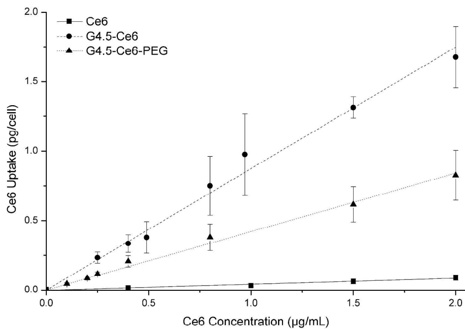
Fig. 3: Cellular uptake of free Ce6 (square), G4.5-Ce6 (round) and G4.5-Ce6-PEG (triangle) incubated with FaDu cells during 24h as function of the PS concentration. 297x207mm (300 x 300 DPI)
