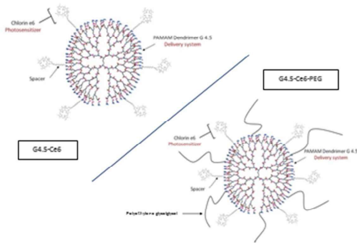
Covalent conjugates between the photosensitizer chlorin e6 and PAMAM G4.5 dendrimers 100x69mm (96 x 96 DPI)
