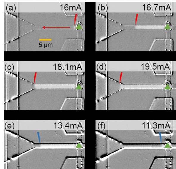
FIG. 2. Evolution of the magnetic configuration along a 2\ \mu m TbCo wire measured under an applied field of 350\ mT using a Kerr microscope and observed as a function of the injected current intensity. (a) A 16\ mA current is injected (red arrow), and a domain is nucleated at the hot spot localized on the defect (green triangle). As we move away from the right defect toward the expansion pad contact on the left, the temperature decreases, creating a temperature gradient along the wire ((a)–(d)). Increasing the current causes the temperature to increase, and the domain wall is shown to move toward the expansion pad—following the thermal gradient motion. ((e) and (f)) When the current is sufficiently reduced, the domain wall will retract back to the nucleation site. When the Co dominant domain expands, the position of the domain wall is marked by a red sign; whereas when the Co dominant domain retracts, the position of the domain wall is marked by a blue sign. The distance between the engineered defect and the pad is 20\ \mu m . Current densities required to propagate are between 2 \times 10^{11}\ A/m^2 and 3 \times 10^{11}\ A/m^2 .
