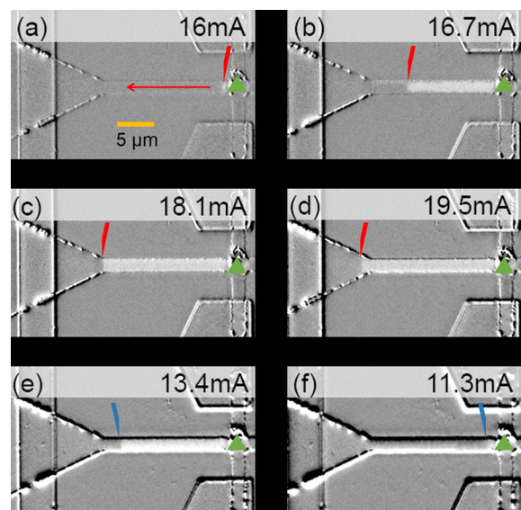
FIG. 2. Evolution of the magnetic configuration along a 2\ \mu\text{m} TbCo wire measured under an applied field of 350\ \text{mT} using a Kerr microscope and observed as a function of the injected current intensity. (a) A 16\ \text{mA} current is injected (red arrow), and a domain is nucleated at the hot spot localized on the defect (green triangle). As we move away from the right defect toward the expansion pad contact on the left, the temperature decreases, creating a temperature gradient along the wire ((a)–(d)). Increasing the current causes the temperature to increase, and the domain wall is shown to move toward the expansion pad—following the thermal gradient motion. ((e) and (f)) When the current is sufficiently reduced, the domain wall will retract back to the nucleation site. When the Co dominant domain expands, the position of the domain wall is marked by a red sign; whereas when the Co dominant domain retracts, the position of the domain wall is marked by a blue sign. The distance between the engineered defect and the pad is 20\ \mu\text{m} . Current densities required to propagate are between 2 \times 10^{11}\ \text{A/m}^2 and 3 \times 10^{11}\ \text{A/m}^2 .
