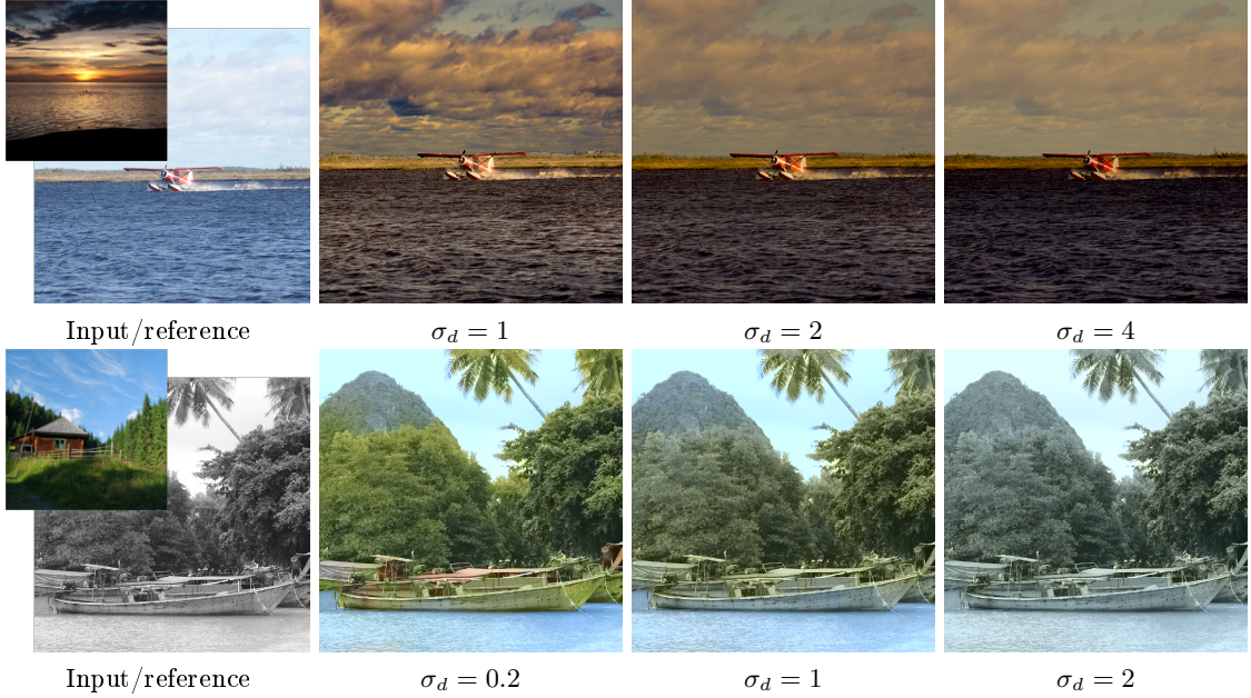
Figure 8: Impact of \sigma_d on transfer functions. Top: color transfer example. When increasing \sigma_d , more and more pixels are considered as similar, resulting in a transfer close to a basic global histogram matching. Bottom: colorization example. As colors are obtained from the weighted average of similar pixels in the reference image, increasing \sigma_d tends to produce a monochrome result.
