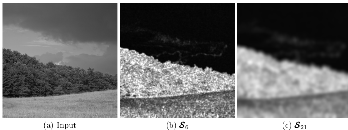
Figure 3: Descriptors. Small scales lead to noisy descriptors (b). Large scales lead to more homogeneous descriptors and smooth sharp texture transitions. For visualization clarity, only the first element of \mathcal{S}_r is shown (i.e. the first value of \mathbf{L}_r^1 ) but the rest of the set presents the same behavior.
