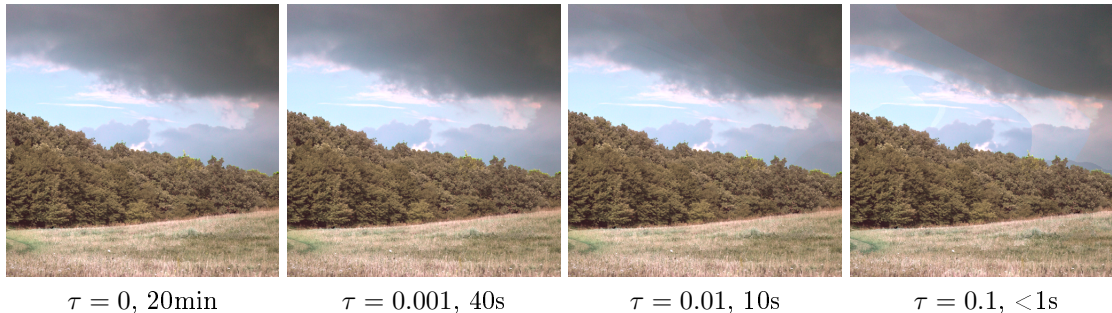
Figure 9: Optimization impact. Color transfer results for increasing \tau values for 512 \times 512 images. The lower \tau , the higher the speed-up and the probability of quantization artifacts. In this example, \tau = 0.1 allows a real-time transfer which can be used for efficient results exploration despite the visual artifacts.
