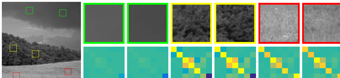
Figure 2: Texture descriptors. Patches taken from several regions of the image in Figure 1 (top) and their respective descriptors computed for the central pixel of the window (bottom). Patches from similar regions have similar descriptors.
