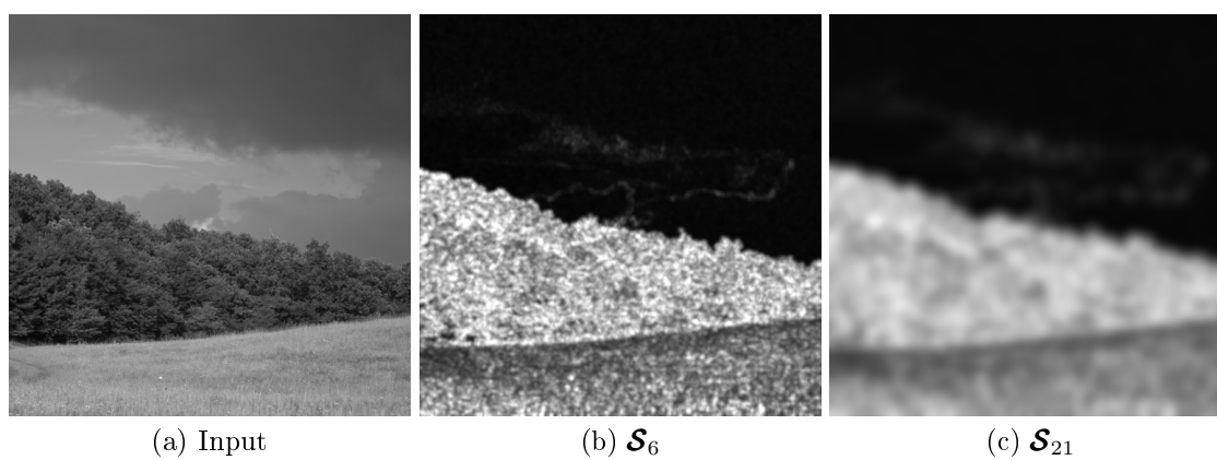
Figure 3: Descriptors. Small scales lead to noisy descriptors (b). Large scales lead to more homogeneous descriptors and smooth sharp texture transitions. For visualization clarity, only the first element of \mathcal{S}_r is shown (i.e. the first value of \mathbf{L}_r^1 ) but the rest of the set presents the same behavior.
