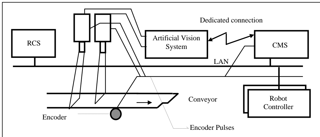
Fig. 1. The robot-based automation system for handling glass plates from a moving conveyor
