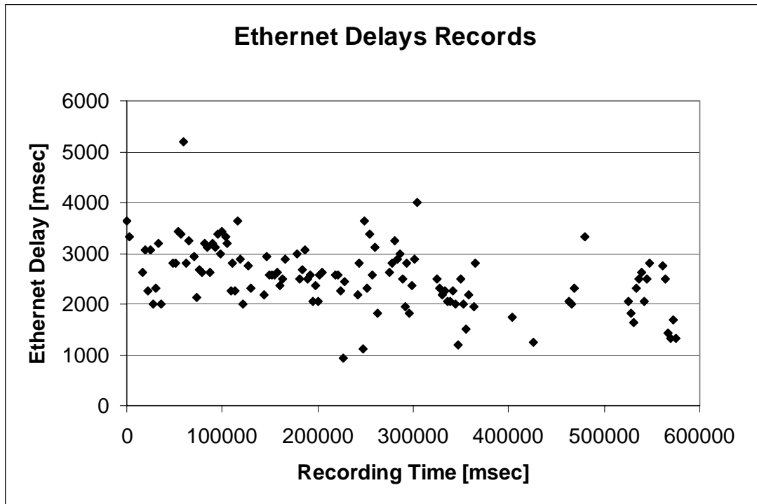
Fig. 2. The experimental results of recording Ethernet Delays over around 10 minutes on the analyzed network.
