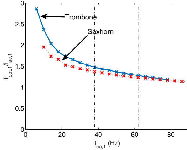
Figure 15: (colour online) Ratio between the predicted oscillation frequency f_{opt,1} and the acoustic resonance frequency f_{ac,1} for different values of the latter. The solid curve plots the results for the trombone, the dotted one for the saxhorn. Vertical dash-dotted lines are the original first resonance frequencies of a trombone (38 Hz) and a saxhorn (62 Hz).
