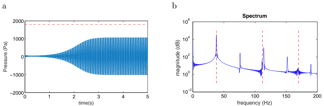
Figure 12: (colour online) Results of simulation of a trombone with a tenor saxophone mouthpiece, modelled as an inward-striking valve with reed resonance frequency f_l = 1 kHz, W = 1 cm, h_0 = 5.10^{-4} m, Q_l = 1.1 , 1/\mu = 4.9 m 2 kg -1 . The blowing pressure p_b = 1800 Pa is slightly above p_{thresh} = 1760 Pa. Left plot (a) shows the blowing pressure (red dashed line) and the mouthpiece pressure (blue solid line). Right (b) plot is the spectrum of the mouthpiece pressure, showing an oscillation frequency f_{thresh} = 37.85 Hz slightly below the first acoustic resonance f_{ac,1} = 38 Hz. Dashed lines represent the resonance frequencies of the bore for comparison.
