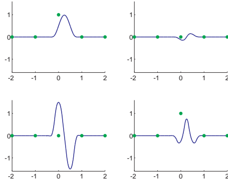
Figure 2: Basic matrix limit function of the non-interpolatory dual Hermite subdivision scheme H_{\bar{\varepsilon}} with \mu = -\frac{1}{2} .
