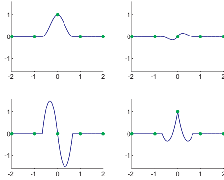
Figure 1: Basic matrix limit function of the interpolatory Hermite subdivision scheme H_{\varepsilon} with \mu = -\frac{1}{2} .
