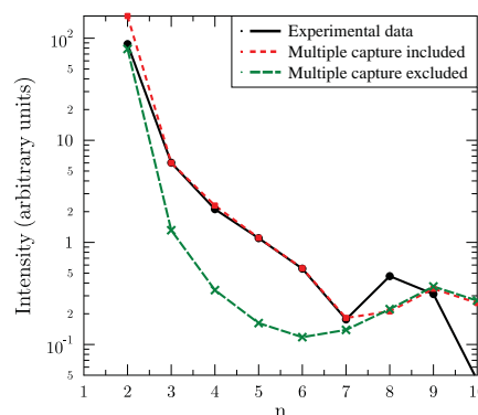
Figure 1. Experimental and calculated X-ray intensities for 1snp \rightarrow 1s^2 transitions in Ar 16+ following electron capture in 15 keV/q Ar 17+ -Ar collisions (see text for details).
