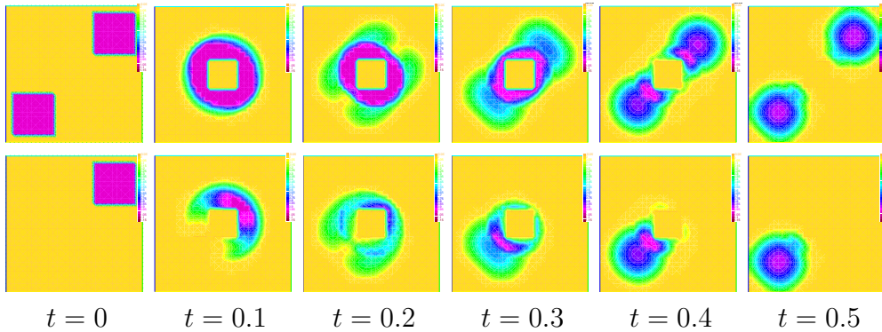
Figure 8: Evolution of two species crossing each other with density constraint and an obstacle. Top row: display of \rho_1 + \rho_2 . Bottom row: display of \rho_1 .
