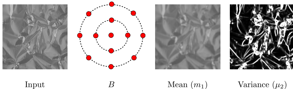
Figure 5: Computation of moment images using structuring element B = \{(1, 4), (2, 8)\} .
