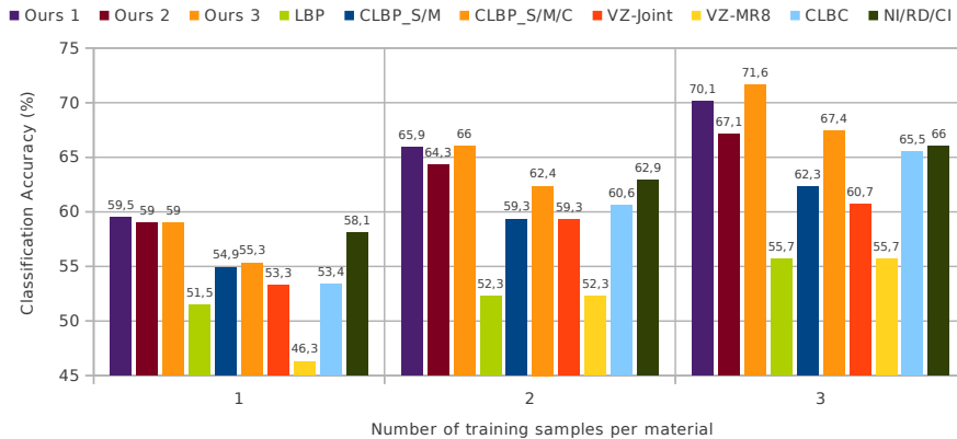
Figure 10: Comparing the best SBP descriptor on single scale (Ours 1), SBP descriptor using limited self-similarity LBP_{8,1}^{riu2} (Ours 2) and multiscale complementary SBP descriptor (Ours 3) with state-of-the-art methods on on KTH-TIPS2b database. Ours 1: SBP_3 with (P, R) = (24, 3) , Ours 2: SBP_3 with (P, R) = (8, 1) and Ours 3: MC\_SBP_4 with (P, R) = \{(8, 1), (8, 2), (8, 3), (8, 4), (8, 5)\} .
