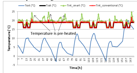
Figure 7 Controlled temperature with conventional method and smart method
