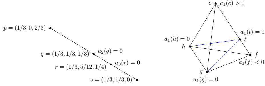
■ Figure 1 Breaking into convex polytopes with constant signs
