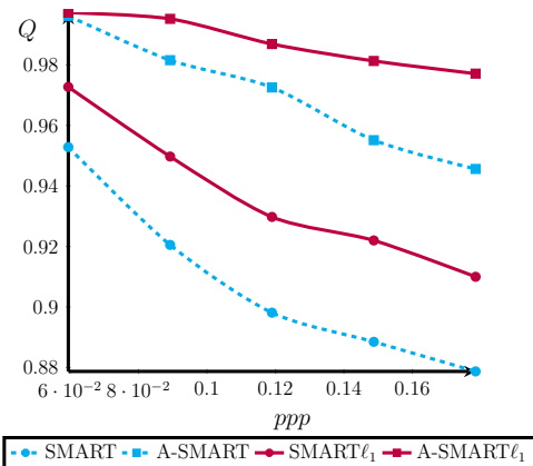
Figure 2. Numerical assessment of the reconstruction quality of \mathbf{x}^{(100)} in a perturbed setting, where y_i is affected by a Gaussian noise of zero mean and standard deviation equal to 0.1y_i . The other parameters are identical to those used in Fig. 1. The performance of the algorithms follows the pattern observed within a non-perturbed setting (see Fig. 1), with the difference that SMART is outperformed by its “sparsity-aware” counterpart.
