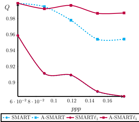
Figure 1. Numerical assessment of the reconstruction quality of \mathbf{x}^{(100)} in an ideal, noise-free scenario for a medium-scale setting (i.e., m = 6724 , n = 99944 ). The results are averaged on 10 experiments. The relaxation parameter \gamma is initially chosen as 0.1, 0.05, 0.4 and 0.8 for SMART, SMART \ell_1 , A-SMART and A-SMART \ell_1 , respectively, and then iteratively adapted following the Armijo rule. We set \tau = \|\mathbf{x}\|_0 (where \mathbf{x} is the ground truth whose non-zero coefficients equal 1) in the “sparsity-aware” versions of (A-)SMART. Regardless of the ppp value, which translates here into sparsity levels growing from \|\mathbf{x}\|_0 = 100 to \|\mathbf{x}\|_0 = 300 , SMART algorithms are outperformed by their accelerated versions. We also notice that, while A-SMART is outperformed by its “sparsity-aware” counterpart, SMART and SMART \ell_1 superimpose.
