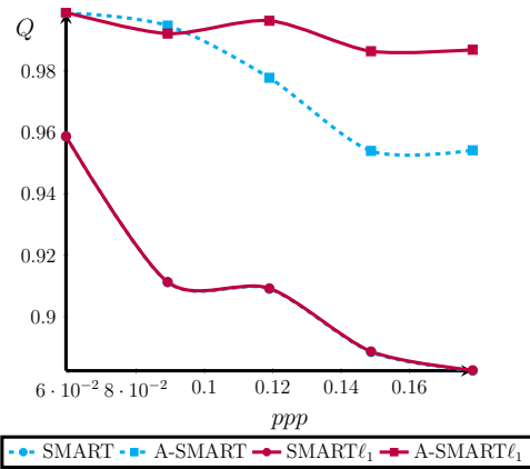
Figure 1. Numerical assessment of the reconstruction quality of \mathbf{x}^{(100)} in an ideal, noise-free scenario for a medium-scale setting (i.e., m = 6724 , n = 99944 ). The results are averaged on 10 experiments. The relaxation parameter \gamma is initially chosen as 0.1, 0.05, 0.4 and 0.8 for SMART, SMART \ell_1 , A-SMART and A-SMART \ell_1 , respectively, and then iteratively adapted following the Armijo rule. We set \tau = \|\mathbf{x}\|_0 (where \mathbf{x} is the ground truth whose non-zero coefficients equal 1) in the “sparsity-aware” versions of (A-)SMART. Regardless of the ppp value, which translates here into sparsity levels growing from \|\mathbf{x}\|_0 = 100 to \|\mathbf{x}\|_0 = 300 , SMART algorithms are outperformed by their accelerated versions. We also notice that, while A-SMART is outperformed by its “sparsity-aware” counterpart, SMART and SMART \ell_1 superimpose.
