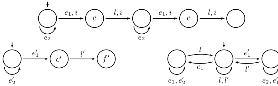
Fig. 4. Three Processes: p (top), p' (bottom left), and arb (bottom right). Only some local boolean variables are represented: c and c' (set to 1 for p and p' in critical section, respectively), and f' set to 1 for p' has finished. The remaining variables are omitted. Effect of the transitions e (resp. e' ) on process p (resp. p' ) depends on the arbiter state. It is therefore split into e_1, e_2 (resp. e'_1, e'_2 ).
