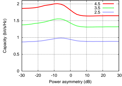
(a) Impact of path loss exponent \alpha
