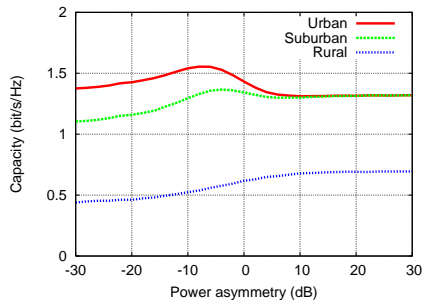
(c) Impact of network density
