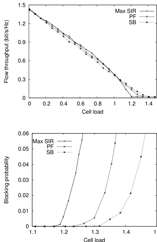
Fig. 10. Flow-level performance for 50% Rayleigh fading.
