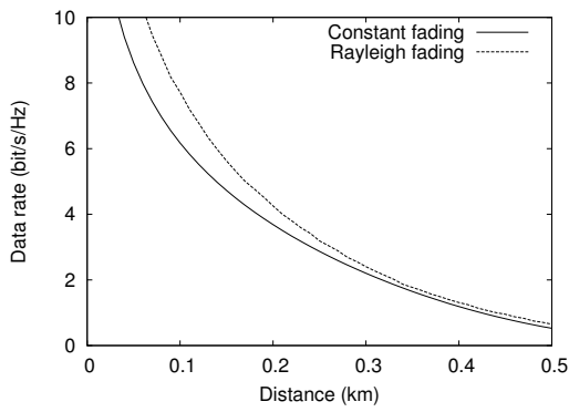
Fig. 4. Feasible rate w.r.t. distance to the BS ( r = 0.5 km).
