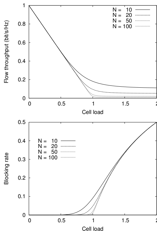
Fig. 7. Flow throughput and blocking rate w.r.t. cell load for various admission thresholds (round-robin scheduler).
