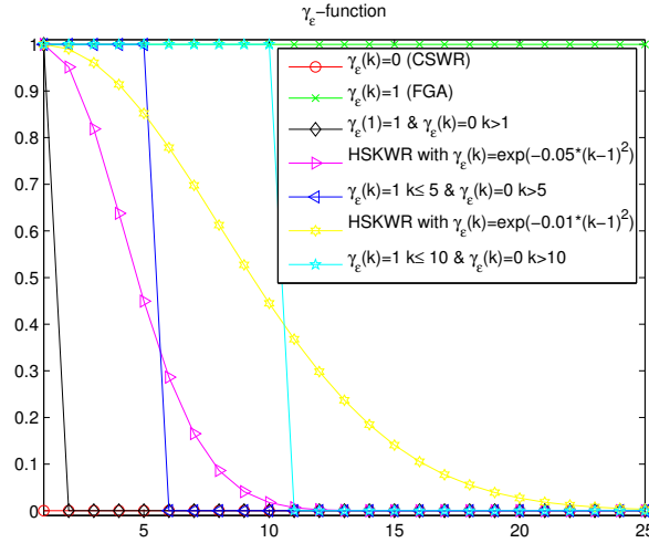
Figure 4.1: Various functions \gamma_\varepsilon .
