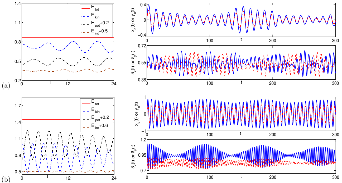
Figure 6: Time evolution of the energies, centre of mass and condensate width in example 4.1 for case II for: (a) s = 0.5 (subdispersion case), (b) s = 1.1 (superdispersion case).
