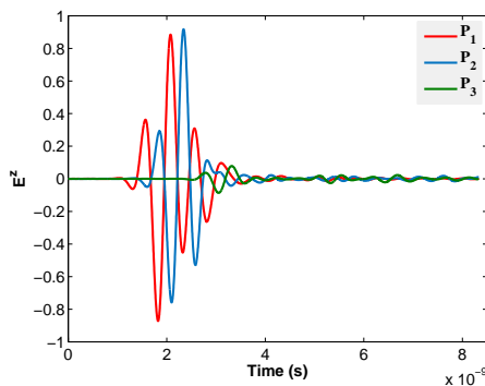
Figure 2: Microwave propagation in head tissues: time evolution of the E^z component of the electric field at selected spatial locations, \vec{P}_1 = (-0.1962, -0.0027, -0.0032) , \vec{P}_2 = (-0.1013, -0.0009, 0.0000) and \vec{P}_3 = (0.0985, -0.0019, -0.0004) .
