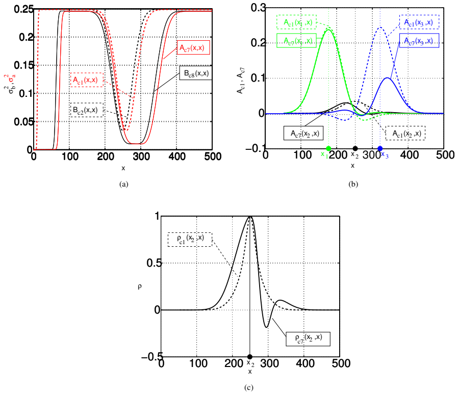
Fig. 15. (a) Error variance at each point for cycle one (dashed curves): analysis \mathbf{A}_{c1} (red) and \mathbf{B}_{c2} (black), and for cycle seven (solid curves): analysis \mathbf{A}_{c7} (red) and \mathbf{B}_{c8} (black). (b) Analysis error covariances in \mathbf{A}_{c1} (dashed curves) and in \mathbf{A}_{c7} (solid curves) for points x_1 = 180 (green), x_2 = x_{\text{obs}} = 250 (black) and x_3 = 320 (blue). (c) Error correlation in \mathbf{B}_{c1} (dashed curve) and \mathbf{B}_{c8} (solid curve) for x_2 = x_{\text{obs}} .
