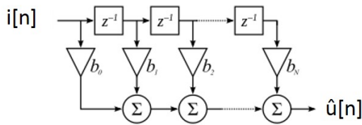
Figure 1: FIR filter
