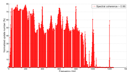
Figure 8: Number of updates according to frequency of the impedance estimation in the passive estimation case.
