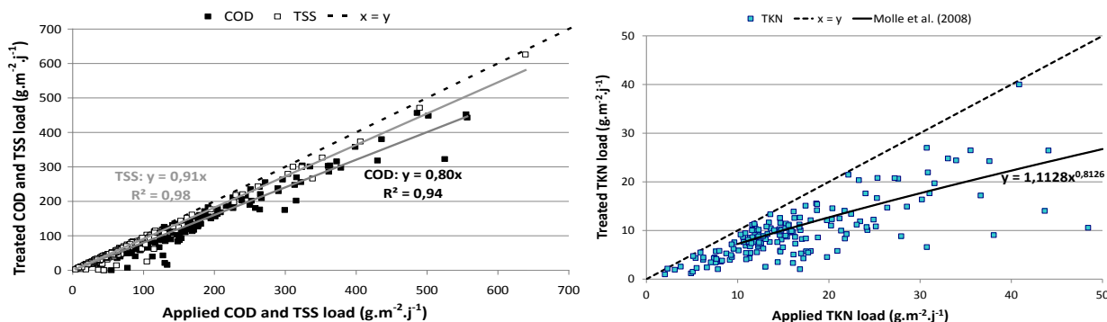
Figure 4. Treated COD, TSS (left) and TKN (right) loads according to the applied COD, TSS and TKN loads on the first stage of VFCW system. N=190 for COD and TSS loads; N =174 for TKN loads
