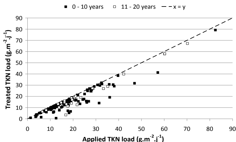
Figure 5. Treated TKN loads according to the applied TKN loads on the first stage of old VFCW plants (aged from 13 to 20 years) according to the age of the plants when the composite samples were made. N =131
