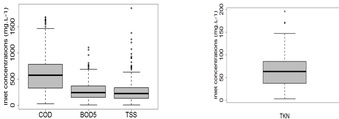
Figure 2. Raw wastewater concentrations (COD, BOD 5 and TSS on the left; TKN on the right) applied on the two-stage VFCW system. N = 394, N = 386, N = 397 and N = 325 for COD, BOD 5 , TSS and TKN, respectively. N: the number of values
