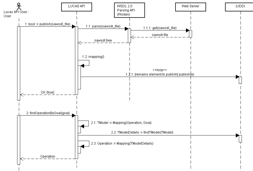
Figure 1 - SAWSDL publishing and registry querying with LUCAS
