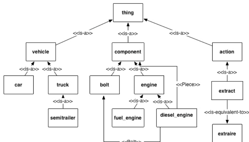
Figure 2 - Exemple ontology
