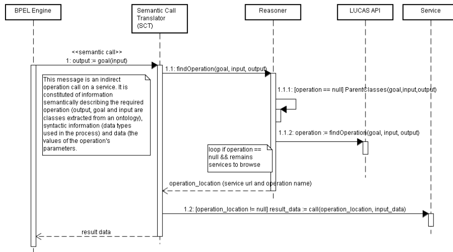
Figure 3 - End to end semantic call handling
