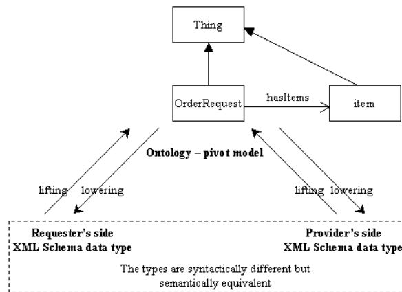
Figure 4 - Ontology as a pivot data model
