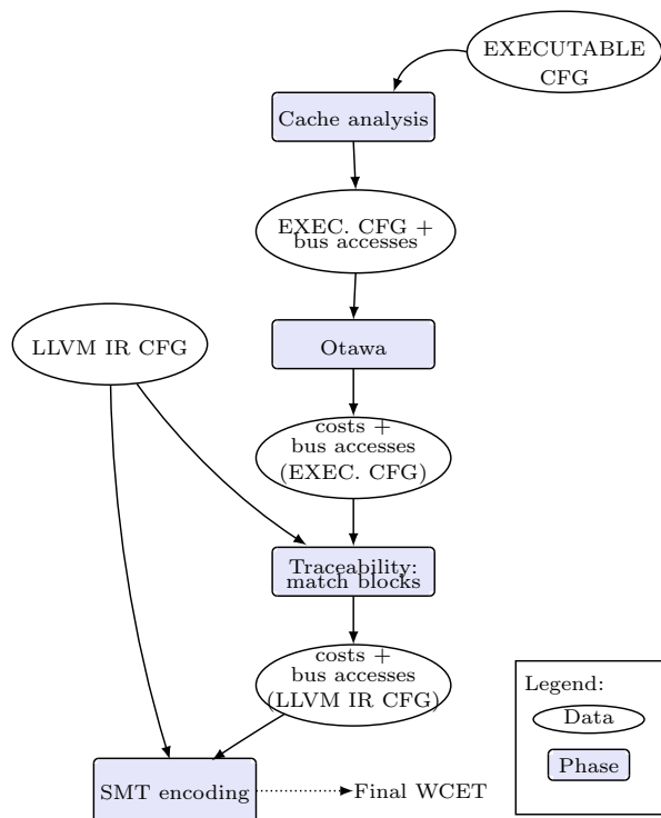
Figure 12: General work flow for realistic timing analysis
