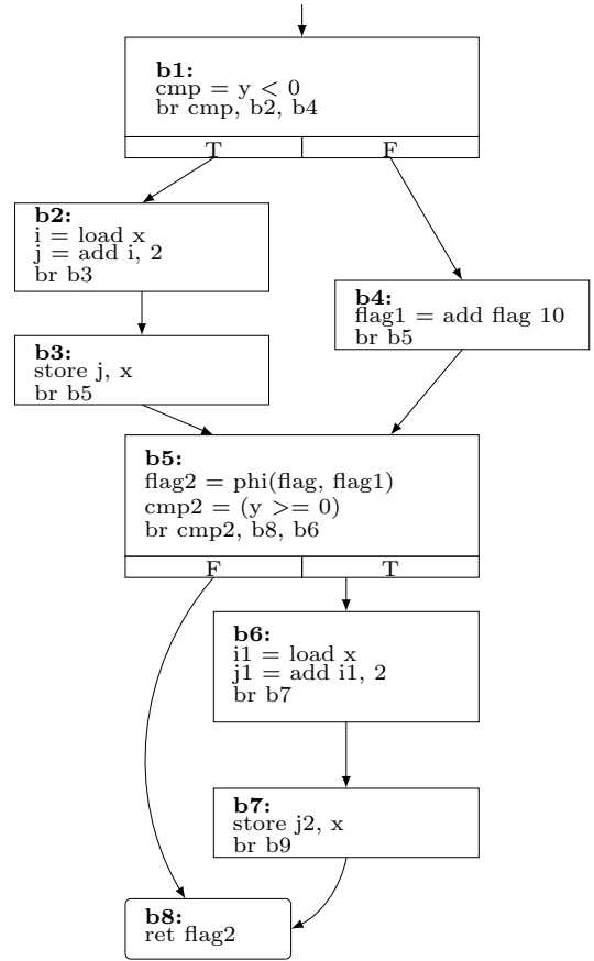
Figure 3: Control-flow graph of Algorithm 2
