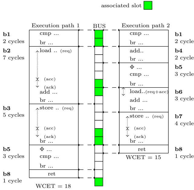
Figure 2: WCET of Algorithm 2 (CFG in Figure 3) with a shared TDMA bus with period \pi = 6 and \sigma = 2
