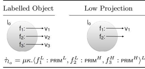
Fig. 5. A Labelled Object and Its Low Projection
