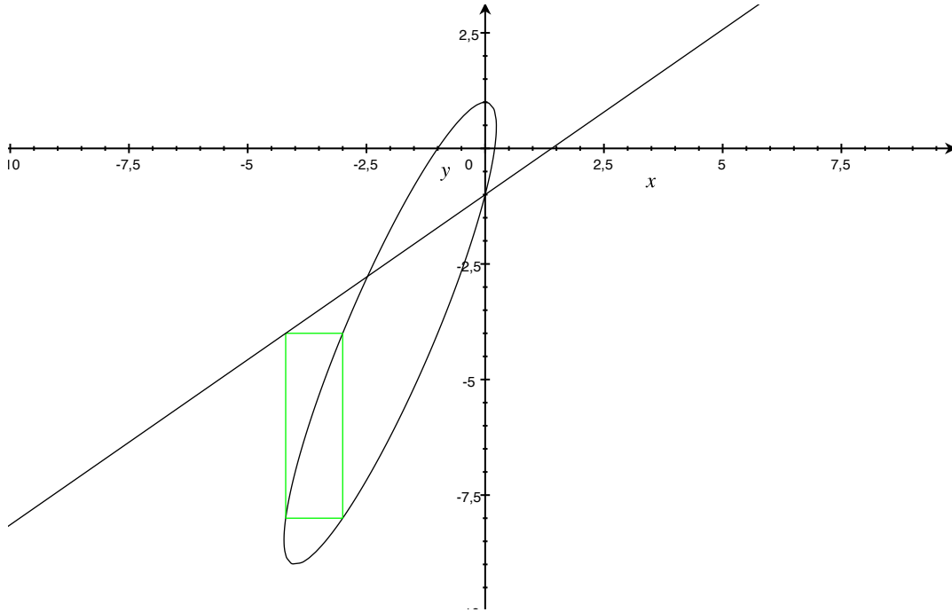
Figure 3: The characteristic variety for the corner problem (117).
