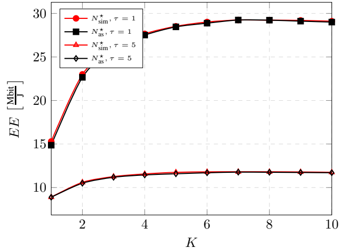
Fig. 5. Energy efficiency achieved by N_{sim}^* and N_{as}^* , as a function of K .
