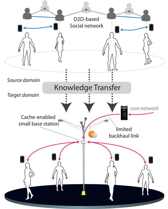
Figure 1: An illustration of the network model which consists of two information systems S^{(S)} and S^{(T)} . Due to the lack of prior information in the target domain, the information extracted from users' social interactions and their ratings in the source domain is transferred to the target domain.
