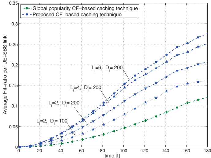
Fig. 2. Time evolution of the hit-ratio per UE-SBS link. |\mathcal{L}_i| = \{2, 4, 6\} UEs, D_i = \{0.22, 0.45\} \cdot |\mathcal{F}| files, B = 1 Gbps, N=100 SBSs.
