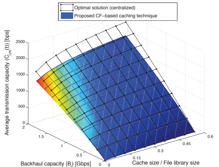
Fig. 5. Average transmission capacity as a function of the normalized cache size D_i/|\mathcal{F}| and backhaul capacity B_i . N = 100 SBSs, r_m^* = 450 Kbps.
