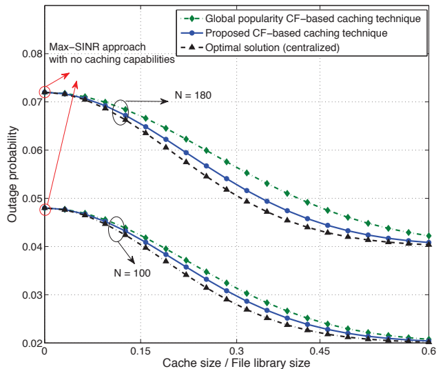
Fig. 3. Average outage probability ( Prob \{C_{i,m}(t) < r_m^*\} ) vs normalized cache size. r_m^* = 450 Kbps, B = 1.8 Gbps.
