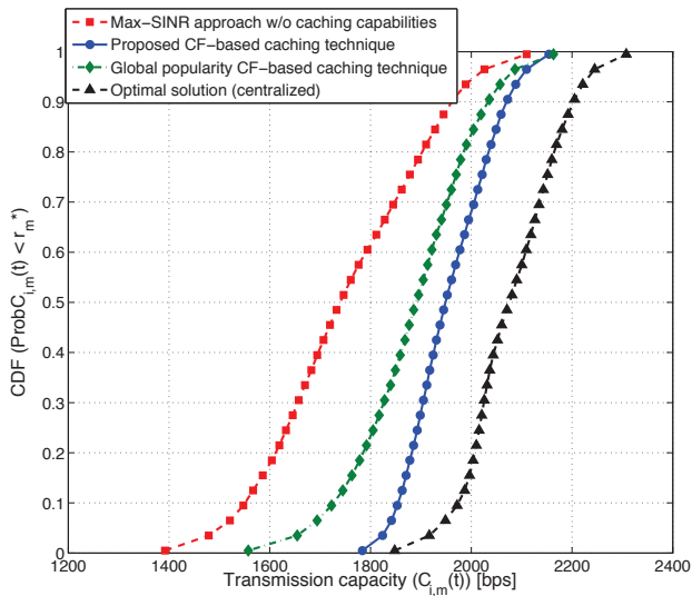
Fig. 4. Cumulative distribution function of the transmission capacity C_{i,m}(t) per UE-SBS link. N = 100 SBSs, r_m^* = 450 Kbps, B = 2 Gbps.
