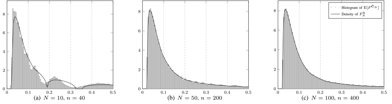
Fig. 2. Density of F_N^R versus histogram of E[F_N^{\hat{C}_N}] for \mathbf{C}_N with [\mathbf{C}_N]_{ij} = .9^{|i-j|} , \mathbf{D}_N = \mathbf{I}_N , \varepsilon = .05 , and u(x) = (1+t)/(t+x) where t = .1 .
