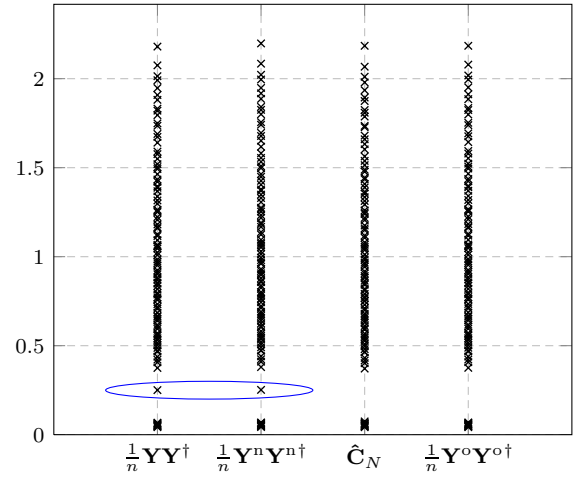
Fig. 1. Eigenvalues of the SCM ( \frac{1}{n}\mathbf{Y}\mathbf{Y}^\dagger ), normalized SCM ( \frac{1}{n}\mathbf{Y}^n\mathbf{Y}^{n\dagger} ), \hat{\mathbf{C}}_N for u = u_S with t = .1 , and the oracle estimator ( \frac{1}{n}\mathbf{Y}^o\mathbf{Y}^{o\dagger} ); N = 100 , c = .2 , \varepsilon_n n = 1 , \mathbf{a}_1 = (\mathbf{a}_1^1, \mathbf{a}_1^2)^\dagger , \mathbf{a}_1^1 \in \mathbb{R}^{10} , \mathbf{a}_1^2 \in \mathbb{R}^{90} , with \mathbf{a}_{1,i}^1 = \sqrt{10} , \mathbf{a}_{1,i}^2 = 0 , such that \|\mathbf{a}_1\|^2 = N ; \mathbf{y}_i = \mathbf{C}_N^{1/2}\mathbf{x}_i with \mathbf{x}_{i,j} standard Gaussian and \mathbf{C}_N = (16/14.50)\text{diag}(\mathbf{c}_1, \mathbf{c}_2) , \mathbf{c}_1 \in \mathbb{R}^{10} , \mathbf{c}_2 \in \mathbb{R}^{90} , with \mathbf{c}_{1i} = 1/16 , \mathbf{c}_{2i} = 1 , such that \text{tr}\mathbf{C}_N = N . Ellipse around the outlier artifact.
