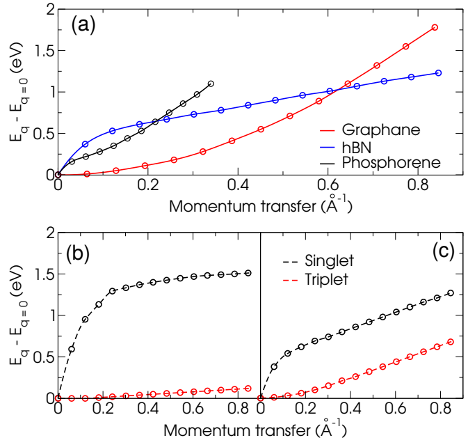
FIG. 3. (a) Calculated dispersion of the lowest-energy bright excitons in graphane and h-BN along \Gamma M and phosphorene along \Gamma X . (b) Singlet and triplet exciton dispersion in h-BN in a two-band model with flat bands and (c) with the real electronic band structure.
