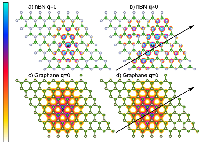
FIG. 2. Electronic distribution of the wavefunction \Psi_{\mathbf{q}}^{\lambda} of the lowest-energy exciton of graphane and h-BN for fixed position of the hole (black sphere) calculated for \mathbf{q} \rightarrow 0 (left) and 0.4 \text{ \AA}^{-1} (right). The black arrow is the direction of \mathbf{q} \neq 0 . White and green spheres represent N and B atoms in h-BN and H and C atoms in graphane.
