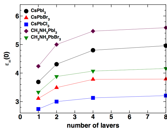
Fig. 6 High frequency dielectric constant at the slab centre \epsilon_{\infty}(0) for \text{CsPbX}_3 ( \text{X} = \text{I}, \text{Br}, \text{Cl} ) and \text{CH}_3\text{NH}_3\text{PbX}_3 ( \text{X} = \text{I}, \text{Br} ) in the [010] direction.
