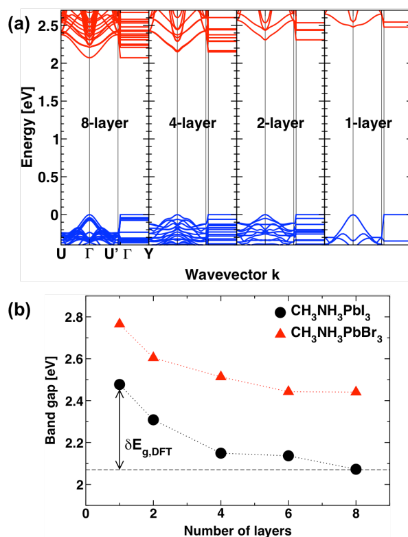
Fig. 4 (a) Band structures for slabs of CH 3 NH 3 PbI 3 with various thicknesses. (b) Band gaps with respect to the slab thickness for CH 3 NH 3 PbX 3 (X = I, Br).
