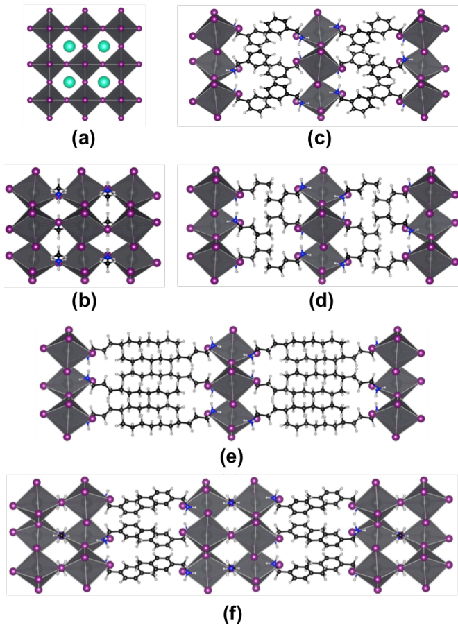
Fig. 2 Structures of (a) all-inorganic \text{CsPbX}_3 ( X = \text{I}, \text{Br}, \text{Cl} ) in the Pm\bar{3}m phase, 63 (b) the 3D HOP \text{CH}_3\text{NH}_3\text{PbI}_3 in the low-temperature Pnma phase, 64 a series of 2D HOP with (c) aromatic organic cation (\text{C}_7\text{H}_{10}\text{N})_2\text{PbI}_4 , 65 (d) and (e) aliphatic organic cation (\text{C}_4\text{H}_{12}\text{N})_2\text{PbI}_4 , 66,67 respectively and (f) the 2D/3D-HOP (\text{C}_{10}\text{H}_{24}\text{N})_2\text{PbI}_3/\text{CH}_3\text{NH}_3\text{PbI}_4 . 68 Pb, Cs, I, N, C and H atoms are depicted in gray, green, purple, blue, black and white, respectively.
