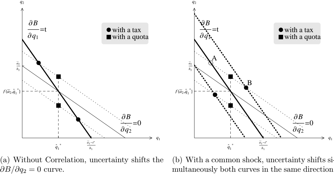
Figure 1: The influence of the uncertainty, surrounding the private value of good 2, on the quantities of good 1 and good 2 with a tax (points) and a quota (squares) without correlation (a) and with correlation (b) for two substitute goods.
