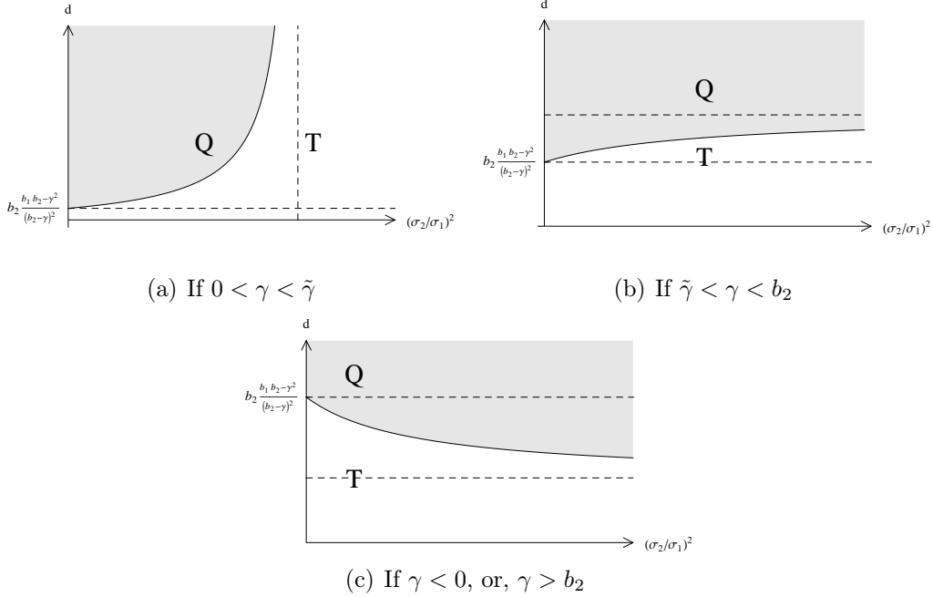
Figure 2: The preferred instrument when the damage depends on total production (specification S) and independent shocks ( \sigma_{12} = 0 ), as a function of the slope of the environmental damage d (y-axis) and the ratio of the variances of the demands \sigma_2^2/\sigma_1^2 (x-axis).
