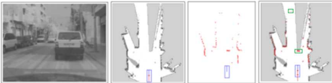
Figure 5. Occupancy grid representation obtained by processing raw lidar data. From left to right: Reference image; static occupancy grid M_{t-1} after applying the SLAM solution; current lidar scan; detection of the moving objects (green bounding boxes).
