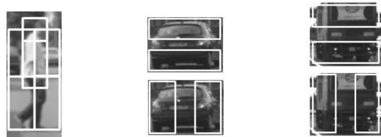
Figure 6. Informative blocks for each object class patch, from left to right: pedestrian, car, and truck. Histograms of gradients are computed over these sparse blocks and concatenated to form S-HOG descriptors. Average size of the descriptors for pedestrians, bikes, cars and trucks are 216, 216, 288 and 288 respectively.
