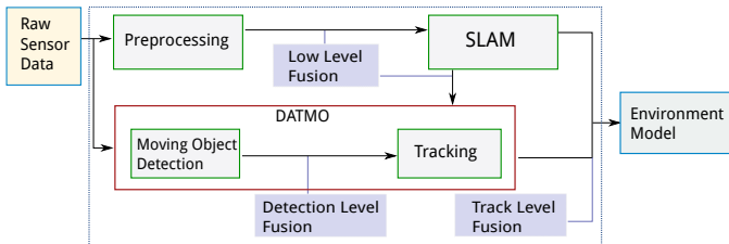
Figure 2. Fusion levels within the SLAM and DATMO components interaction.
