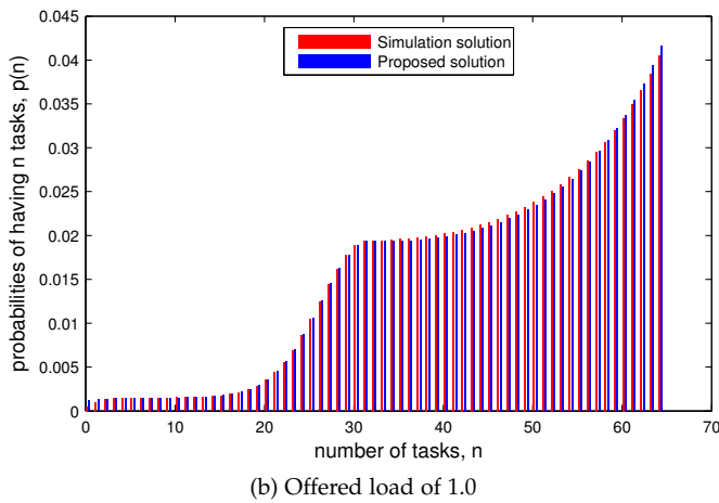
Fig. 5: Distributions of the number of tasks, p(n) , produced by the exact and our approximate solutions.
