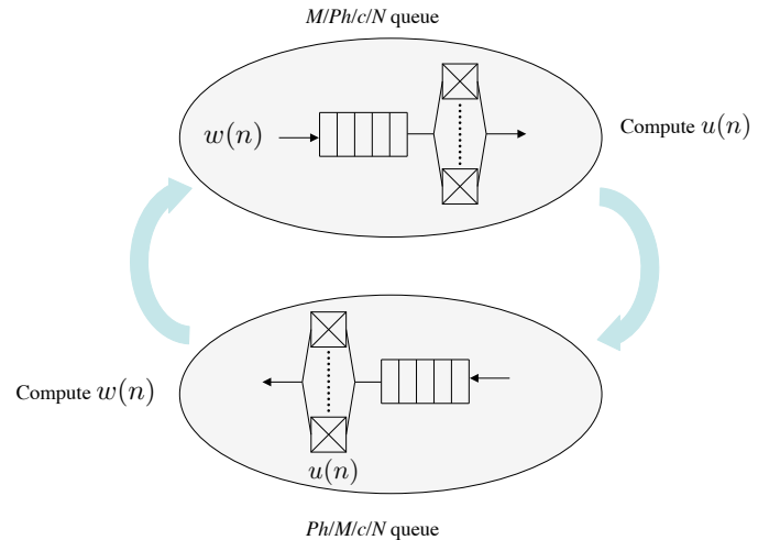
Fig. 4: Schematic view of the approximate solution.
