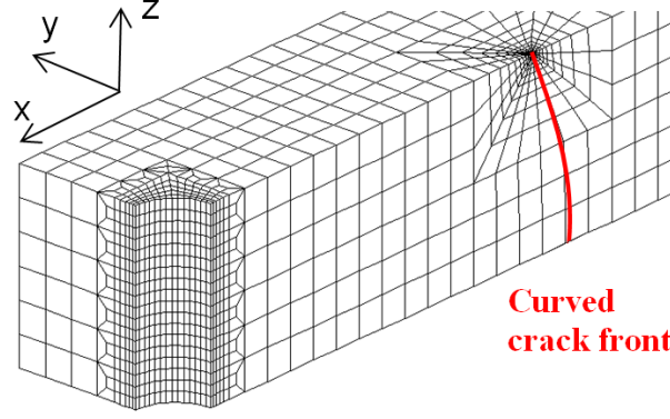
Figure 11. 3D mesh for the finite element simulation of the DCDC sample. Due to symmetry, only 1/8^{\text{th}} of the specimen is meshed. The crack front is curved to a parabolic front with terminal angle \alpha and the mesh is densified at the corner point singularity.
