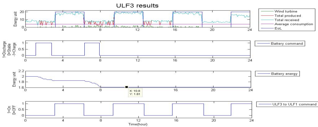
Fig. 4: ULF3 optimization results.
