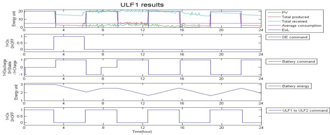
Fig. 2: ULF1 optimization results.
