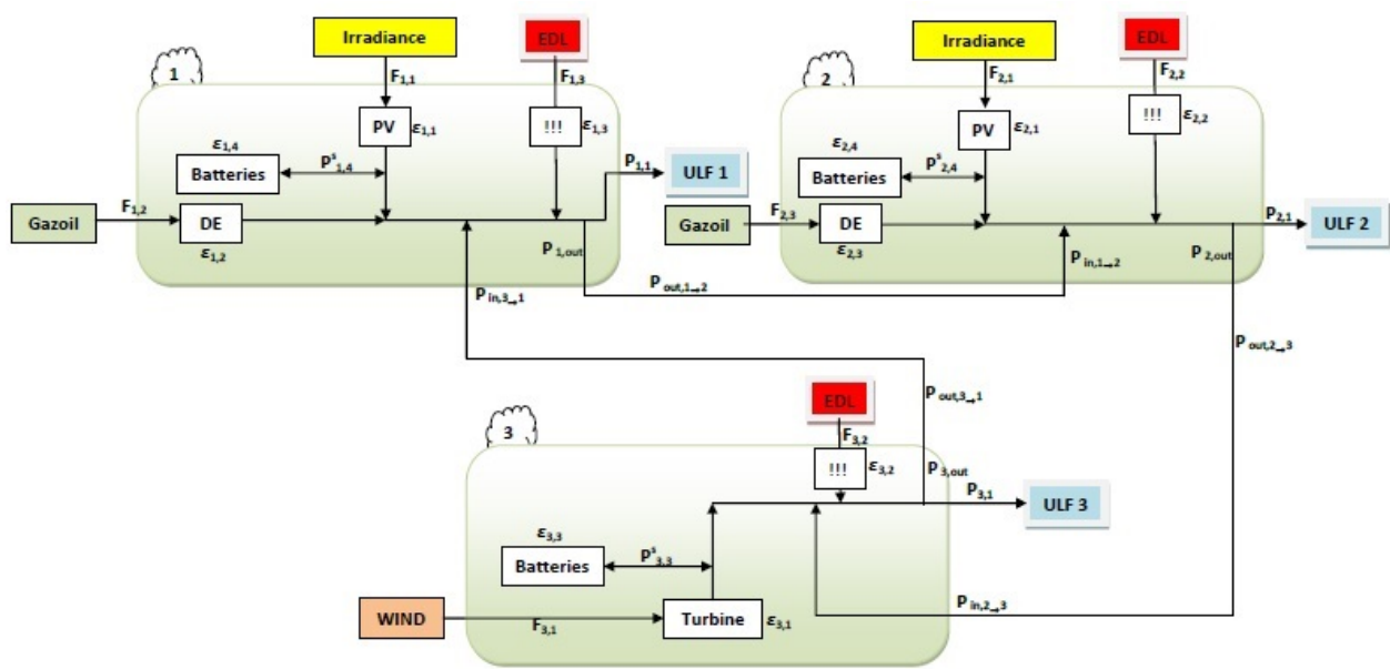
Fig. 1: The ULF grid and the interaction between each energy hub.
