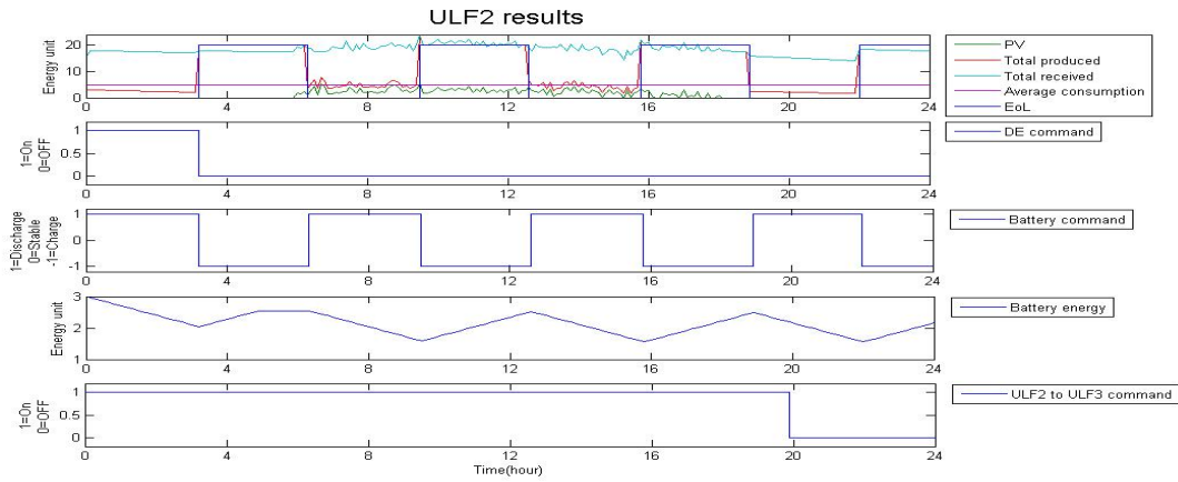
Fig. 3: ULF2 optimization results.
