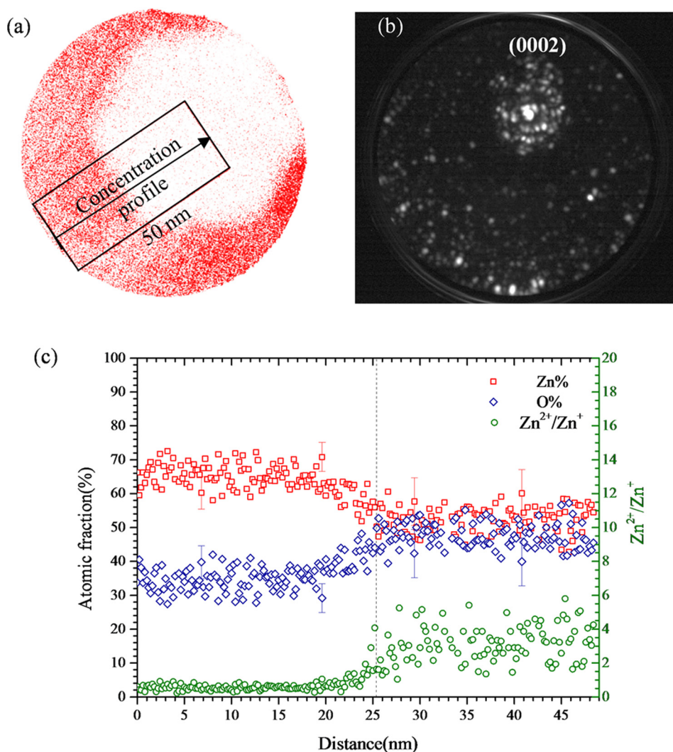
FIG. 7. (a) Distribution of Zn + ions at LPE = 5 nJ, (b) field ion microscopy image of the same nanowire presenting the existence of a crystallographic pole at the place where the highest field is seen (c) concentration profile for a 3D selected zone shown in (a). For clarity reason, only few error bars are shown.
