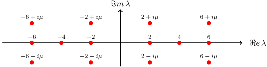
Figure 7: Set \Lambda for \kappa_\sigma = -2 . This configuration is characteristic of the case \kappa_\sigma \in (-3, -1) .
