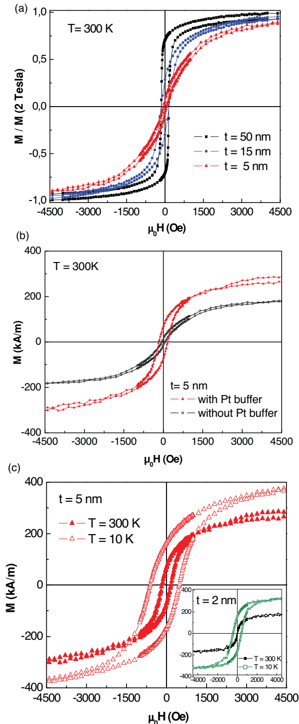
FIG. 7. (Color online) (a) In-plane magnetic hysteresis loops for \alpha - \text{Al}_2\text{O}_3/\text{MnFe}_2\text{O}_4(111) thin films (50, 15, and 5 nm) at T = 300 K. (b) In-plane magnetic hysteresis loops for an \alpha - \text{Al}_2\text{O}_3/\text{MnFe}_2\text{O}_4(111) (5 nm) thin film and an \alpha - \text{Al}_2\text{O}_3/\text{Pt}(20 \text{ nm})/\text{MnFe}_2\text{O}_4(111) (5 nm) thin film at T = 300 K. (c) In-plane magnetic hysteresis loops for an \alpha - \text{Al}_2\text{O}_3/\text{Pt}(20 \text{ nm})/\text{MnFe}_2\text{O}_4(111) (5 nm) (2 nm, in inset) thin film at T = 300 K and 10 K.
