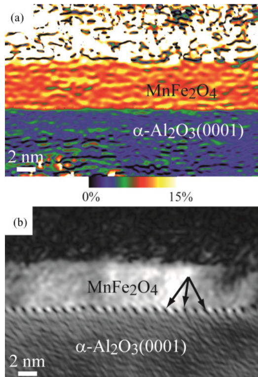
FIG. 5. (Color online) (a) Strain map along the growth direction calculated from the HRTEM image using the GPA method. (b) Amplitude image with regularly spaced contrasts (some of them are indicated by arrows) corresponding to the misfit dislocations.
