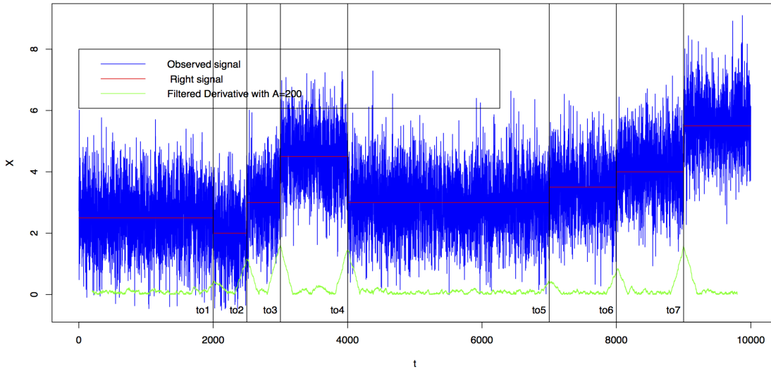
Figure 2: A graph of the Filtered Derivative function
