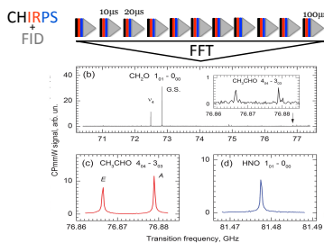
Typical time sequence with segmented chirps to monitor the products formed in the pyrolysis of CH 3 CH 2 ONO. Here a broadband 7 GHz chirp covering 70.4–77.4 GHz (black) is used in combination with 20 MHz chirps centered on relevant known transitions for CH 3 CHO (red) and HNO (blue). Ref. [3]
