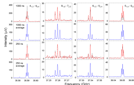
Several rotational transitions of dimethyl ether (J K a ,K c - J K a ,K c ' ) over the 34–40 GHz frequency range are shown to illustrate the effects of collisional dephasing on signal intensities. The top row of spectra was taken with chirp duration of 1000 ns, and a clear asymmetry exists in the line intensities between up- (red trace) or down-swept (black) frequencies. This asymmetry is less severe in spectra obtained with a 250 ns chirp duration (middle row) or shorter. Averaging up- and down-chirped spectra can compensate for the dephasing effects, as shown in rows two and four (blue traces) for the 1000 and 250 ns spectra, respectively. Ref. [5]
