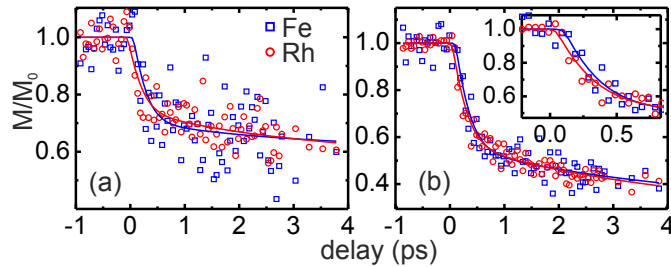
FIG. 2. Element resolved demagnetization dynamics of FeRh (Fe: blue open squares, Rh: red open circles) obtained by TR-XUV-TMOKE. The reduced magnetization ( M/M_0 ) after excitation with a) 11 mJ/cm 2 and b) 16 mJ/cm 2 . The inset in b) shows a zoom to the initial drop of the signal. Fe demagnetization is delayed with respect to Rh by approximately 60 fs.
