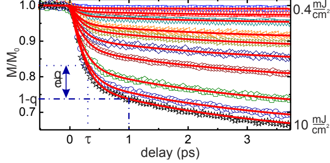
FIG. 3. TR-MOKE demagnetization traces of FeRh for various fluences ( 0.4 - 10 \text{ mJ/cm}^2 ). The solid line (red) is a fit using the M3TM-model, where only the spin-flip rate and the excitation strength is allowed to vary. The demagnetization time \tau (dotted line) referenced to the quenching q (defined as the loss of magnetization at 1 ps, dashed-dotted line) is visualized for the trace with the highest fluence ( 10 \text{ mJ/cm}^2 ).
