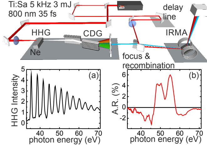
FIG. 1. Sketch of the CITIUS HHG light source. The 3 mJ/pulse Ti:Sapphire laser output is split in two branches: 2 mJ/pulse are used for HHG and 1 mJ/pulse for sample excitation (IR pump). The proper harmonic is selected by means of a time preserving monochromator based on conical diffraction gratings (CDG) and refocalized onto the sample. The IR pump is recombined with the HHG light in the experimental chamber IRMA on the sample in an almost collinear geometry. a) The higher harmonics spectrum from Ne after the monochromator captured with a photodiode and b) the normalized magnetic asymmetry ratio (A.R.), namely the difference of both field directions divided by their sum, for the T-MOKE like configuration in the IRMA setup.
