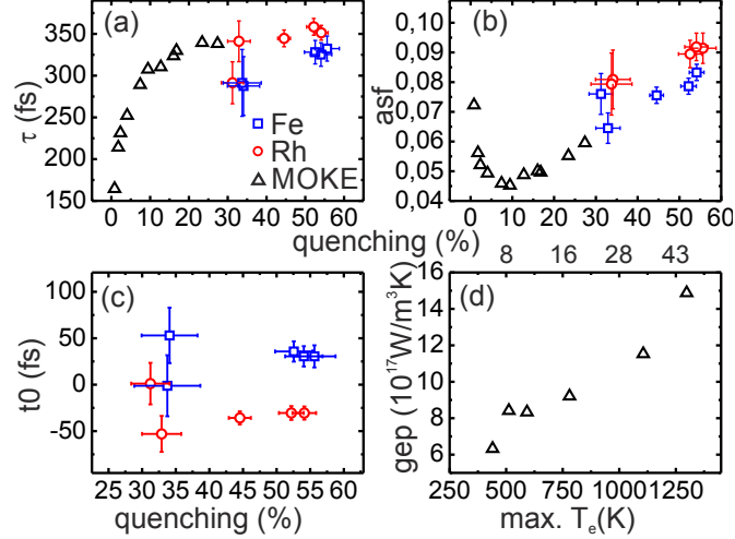
FIG. 4. Fit parameters from the M3TM for element resolved measurements, Rh (red open circles), Fe (blue open squares) and for TR-MOKE and the transient optical response (black open triangles, errorbars are within the symbol size). a) The demagnetization time \tau and the b) spin-flip rate a_{sf} which is a key parameter for describing the demagnetization time and the quenching versus fluence. c) The difference in t_0 for the element resolved demagnetization times shows that Fe starts delayed by about 60 fs with respect to Rh for various fluences. Errorbars for lower fluence appear bigger due to a lower signal and a nearly constant noise level in all measurements. d) The electron phonon coupling g_{ep} is not constant as a function of the maximum electronic temperature or the resulting calculated quenching.
