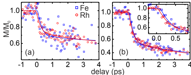
FIG. 2. Element resolved demagnetization dynamics of FeRh (Fe: blue open squares, Rh: red open circles) obtained by TR-XUV-TMOKE. The reduced magnetization ( M/M_0 ) after excitation with a) 11 mJ/cm 2 and b) 16 mJ/cm 2 . The inset in b) shows a zoom to the initial drop of the signal. Fe demagnetization is delayed with respect to Rh by approximately 60 fs.
